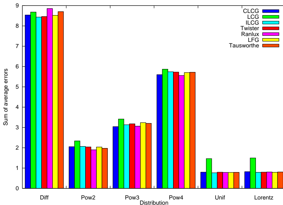
Figure B.2: Sums of average errors: Non-uniform discrete random variables
