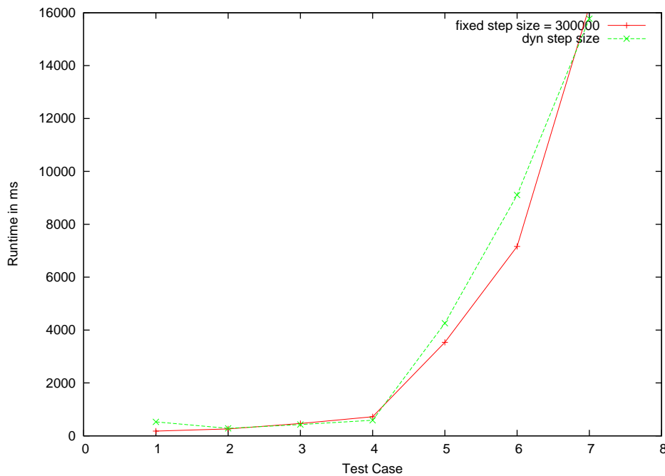
Figure C.2: Runtime: dynamic and fixed sample size step
